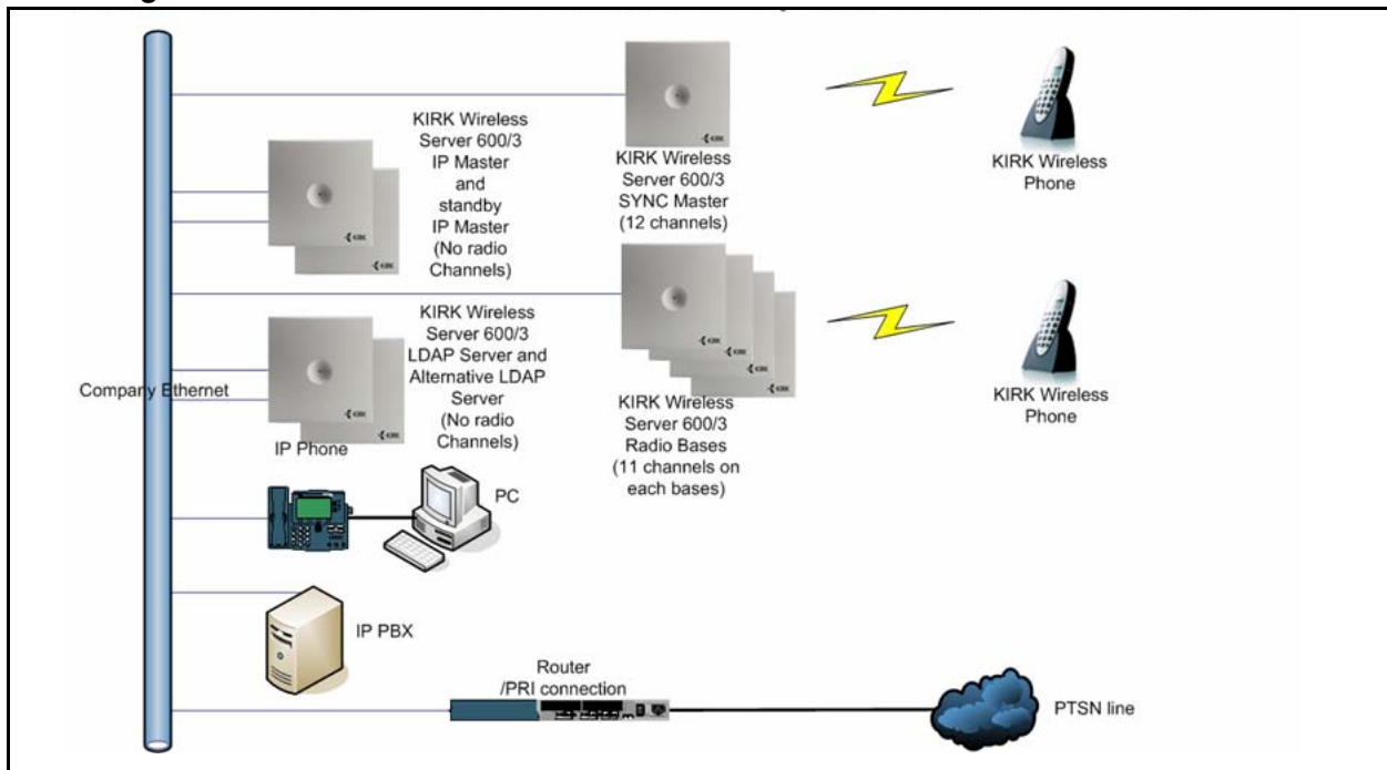
Figure 91 KWS600v3 Multi-cell installation with Alternative LDAP Server
